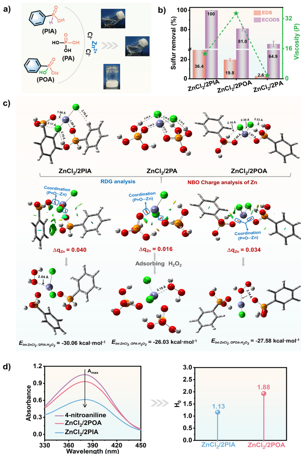
Fig. 2 (a) Schematic of PDES 2X/ \text{ZnCl}_2 (X = PIA, PA, and POA) synthesis. (b) The relationship between extraction/catalytic performance and viscosity. (c) Gradient isosurface ( s = 0.35 a.u.) of optimal PDESS, and adsorption energy analysis with the \text{H}_2\text{O}_2 oxidant. (d) Hammett function calculation using 4-nitroaniline ( \text{pK}(\text{I})_{\text{aq}} = 0.99 ) as the indicator.
