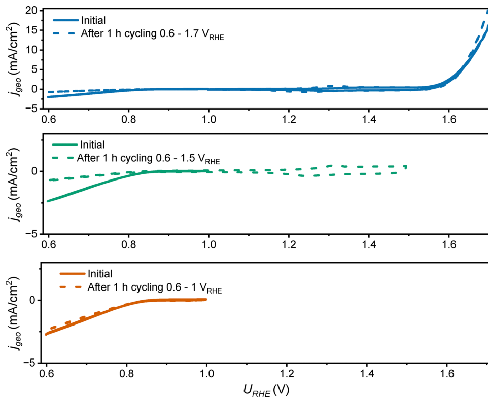
Fig. 10 Geometric electrochemical activity of co-precipitated \text{NiCo}_2\text{O}_4 before (full line), and after (dashed line) cycling for 1 h between 0.6\text{ V}_{\text{RHE}} and three different anodic limits of 1.7\text{ V}_{\text{RHE}} , 1.5\text{ V}_{\text{RHE}} , and 1\text{ V}_{\text{RHE}} at 500\text{ mV s}^{-1} , as described in the figure labels. Results collected in 0.1\text{ M KOH} , \text{O}_2 bubbling at 150\text{ mL min}^{-1} , at 1600\text{ RPM} , 10\text{ mV s}^{-1} , and a loading of 76\text{ }\mu\text{g}_{\text{NiCo}_2\text{O}_4}\text{ cm}^{-2} .
