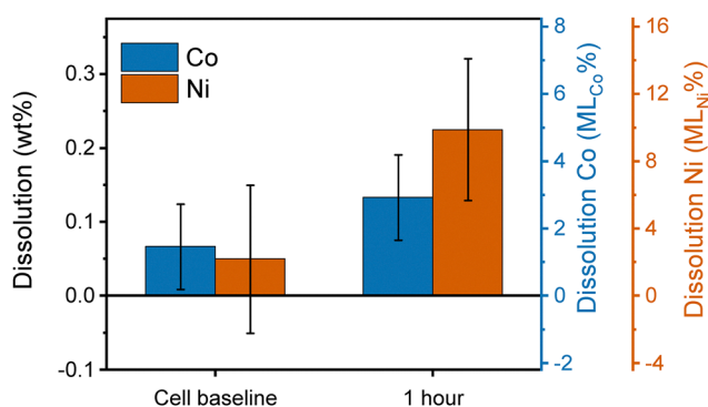
Fig. 11 ICP-MS results after acidification of 150\text{ mL} of the 0.1\text{ M KOH} electrolyte employed in rotating disk electrode configuration to study co-precipitated \text{NiCo}_2\text{O}_4 . Cell baseline taken after assembling the RDE configuration, and 1 hour is taken after cycling between 0.6\text{--}1.7\text{ V}_{\text{RHE}} for 1 hour at 500\text{ mV s}^{-1} without any RDE rotation and employing an anion exchange membrane to separate the counter electrode from the working electrode at a loading of 76\text{ }\mu\text{g}_{\text{NiCo}_2\text{O}_4}\text{ cm}^{-2} . Calculations of Ni and Co dissolved monolayers are based on 0.076\text{ Co atoms per }\text{\AA}^2 derived from the work of Zasada et al. , 158 and the BET surface area of Co-precipitated \text{NiCo}_2\text{O}_4 ( 107\text{ m}^2\text{ g}^{-1} ). Dissolved Ni in %ML is the ratio between dissolved Ni atoms and total available surface Ni atoms in the RDE catalyst layer as described in the SI.
