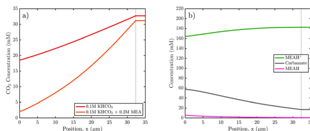
Fig. 8 Simulated boundary-layer concentration profiles at an applied potential of -1.5 V vs. SHE, where the zero coordinate corresponds to the Ag cathode surface. (a) Comparison of the dissolved \text{CO}_2 concentration profile in 0.1 M \text{KHCO}_3 electrolyte with and without 0.2 M MEA additive. (b) MEA, \text{MEA}^+ , and carbamate concentration profiles in 0.1 M \text{KHCO}_3 + 0.2 M MEA electrolyte, showing the depletion of \text{MEA}^+ and accumulation of MEA and carbamate relative to their respective bulk values. Carbamate concentration is elevated due to the reaction of locally generated MEA with aqueous \text{CO}_2 , causing the result in (a). 17 Reproduced with permission from ref. 17, copyright 2023 American Chemical Society.
