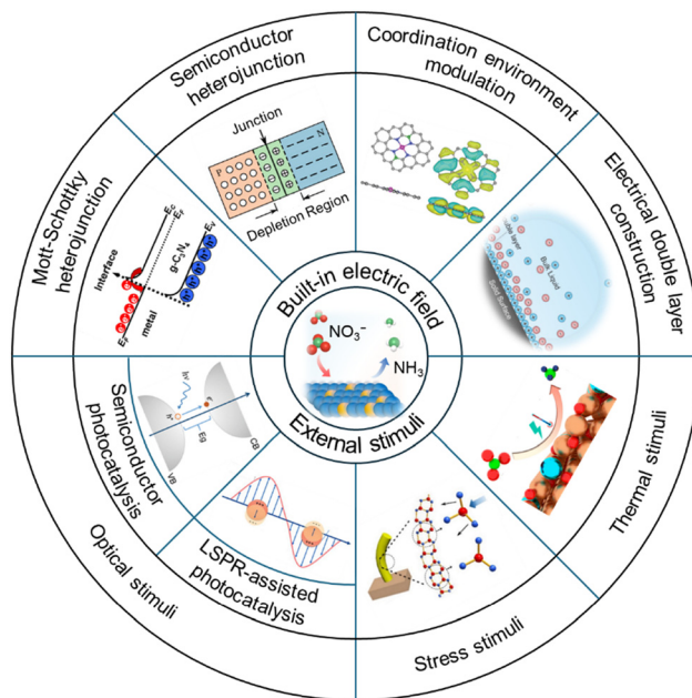
Fig. 1 Schematic of a built-in electric field/external stimuli-assisted \text{NO}_x\text{RR} .
