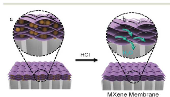
Fig. 7 (a) 2D MXene nanosheets based membrane with colloidal \text{Fe}(\text{OH})_3 (yellow spheres). (b) Hydrochloric acid solution (HCl) treatment to remove the \text{Fe}(\text{OH})_3 nanoparticles from the synthesized MXene. Reproduced from ref. 45 with permission from Wiley, copyright 2017.
