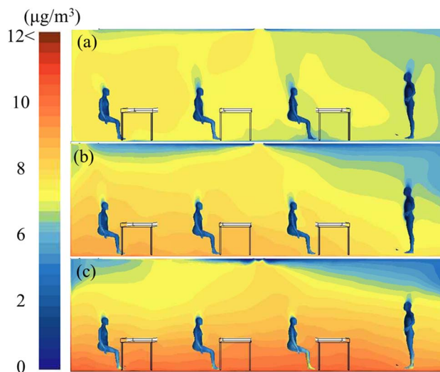
Fig. 6 Distribution of SOA concentrations under mixing ventilation with an inlet air temperature of (a) 14 °C (case 4, cooling), (b) 38 °C (case 5, heating), (c) 50 °C (case 6, heating).
