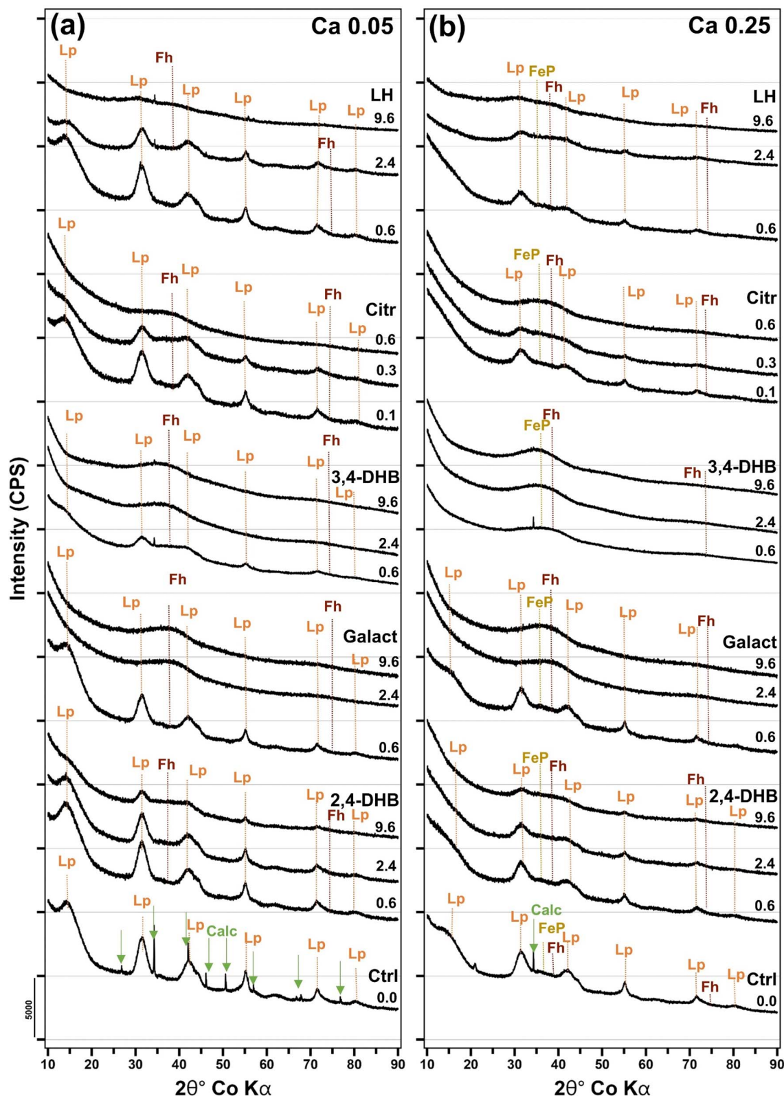
Fig. 4 X-ray diffraction patterns of Fe(III)-precipitates from the Ca electrolyte with a (P/Fe) init of 0.05 (a) and 0.25 (b). Peak positions are indicated for lepidocrocite (Lp, orange), 2-line ferrihydrite (Fh, brown), amorphous Fe(III)-phosphate (FeP, olive) and calcite (Calc, green). For the Na 0.05 and Na 0.25 treatments, the XRD data are shown in Fig. S7.†
