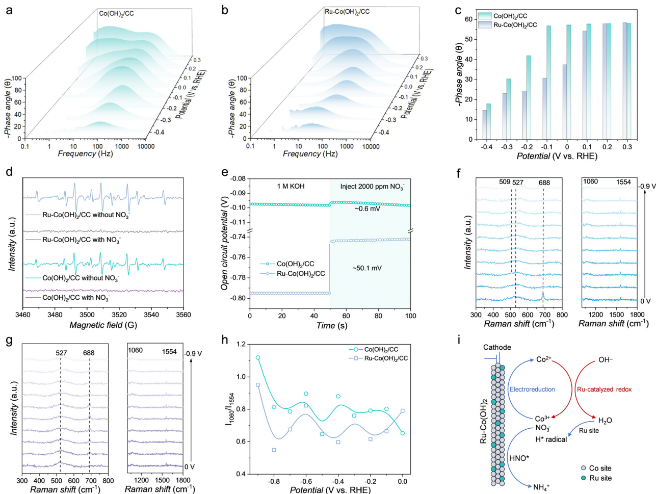
Fig. 3 Operando characterization and the mechanism of the phase transition. (a) Bode phase plots of (a) Co(OH) 2 /CC and (b) Ru–Co(OH) 2 /CC at varied potentials in Ar-saturated 1 M KOH solution with 2000 ppm NO 3 − . (c) Phase peak angles of Co(OH) 2 /CC and Ru–Co(OH) 2 /CC at 0.3 to −0.4 V vs. RHE. (d) Quasi in situ EPR trapping of hydrogen radicals. (e) OCP curves of Ru–Co(OH) 2 /CC and Co(OH) 2 /CC in Ar-saturated 1 M KOH and 2000 ppm NO 3 − was injected subsequently. In situ Raman spectra of (f) Ru–Co(OH) 2 /CC and (g) Co(OH) 2 /CC at different applied potentials in Ar-saturated 1 M KOH solution with 2000 ppm NO 3 − . (h) I 1060/1554 for Ru–Co(OH) 2 /CC and Co(OH) 2 /CC at different applied potentials. (i) Proposed mechanism of NH 3 synthesis from the electrochemical reduction of NO 3 − over Ru–Co(OH) 2 /CC.
