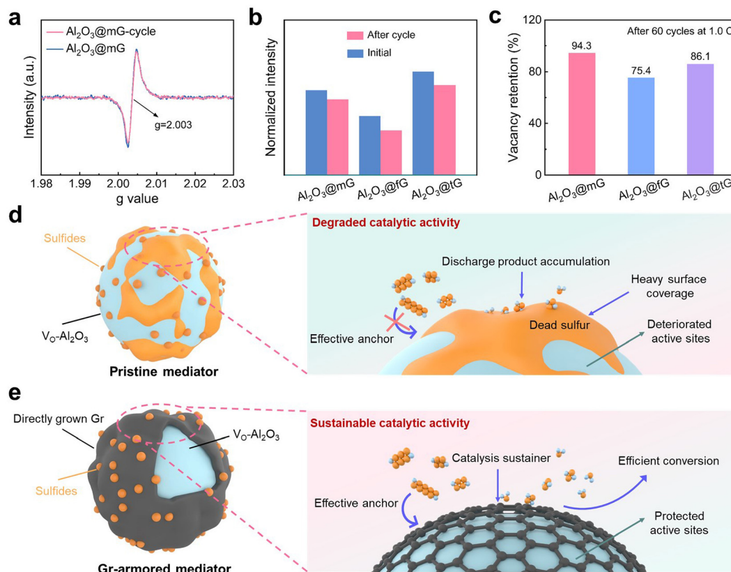
Fig. 3 Mechanism of active site failure and protection. (a) Ex situ EPR spectra of \text{Al}_2\text{O}_3 @mG. (b) EPR intensity of different \text{Al}_2\text{O}_3 @G samples before and after cycling. (c) Corresponding vacancy retention rates after 60 cycles at 1.0 C. Schematic illustrating the evolution of vacancy sites on (d) the pristine mediator and (e) the graphene-armed mediator during the electrochemical process.
