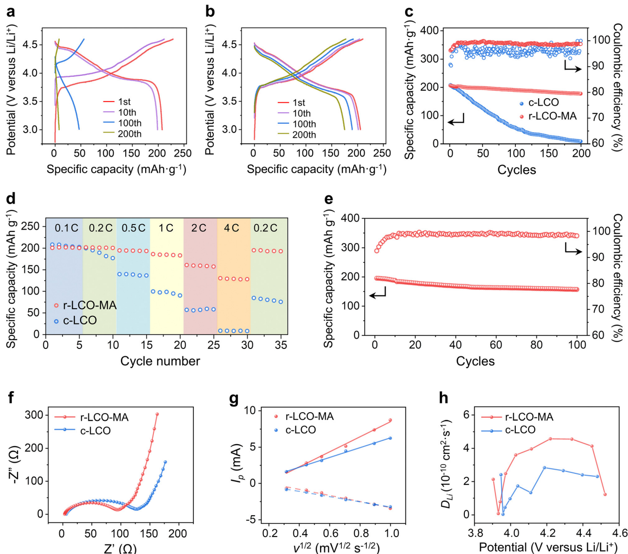
Fig. 3 Electrochemical performance of resynthesized LCO cathode. (a) and (b) Charge–discharge profiles at different cycles for c-LCO, and r-LCO-MA. (c) Cycling stability of c-LCO (blue spot) and r-LCO-MA anode (red spot) at 0.2 C. (d) Rate capacity of c-LCO (blue spot) and r-LCO-MA anode (red spot). (e) Cycling stability of the full-cell LIB with r-LCO-MA cathode and graphite anode at 0.2 C. (f) Comparison of Li + diffusion coefficients of r-LCO-MA (red line) and c-LCO cathodes (blue line). (g) and (h) Li + diffusion coefficient of r-LCO-MA (red line) and c-LCO cathodes (blue line) during the charging and discharging process by GITT.
