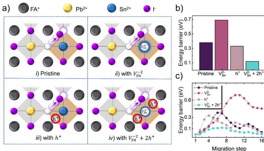
Fig. 4 (a) Theoretical model of the iodide migration pathway in a \text{FAPb}_{0.5}\text{Sn}_{0.5}\text{I}_3 lattice under four scenarios: (i) \text{V}_\text{I}^+ ( i.e. the pristine case), (ii) \text{V}_\text{I}^+ and \text{V}_\text{Sn}^{2-} , (iii) \text{V}_\text{I}^+ and \text{h}^+ , and (iv) \text{V}_\text{I}^+ , \text{V}_\text{Sn}^{2-} , and 2\text{h}^+ . (b) The energy barriers for iodide migration of each proposed scenario. (c) Relative energy landscapes of the system during iodide migration, the x-axis represents the iodide migration step during its transition towards an adjacent \text{V}_\text{I}^+ .
