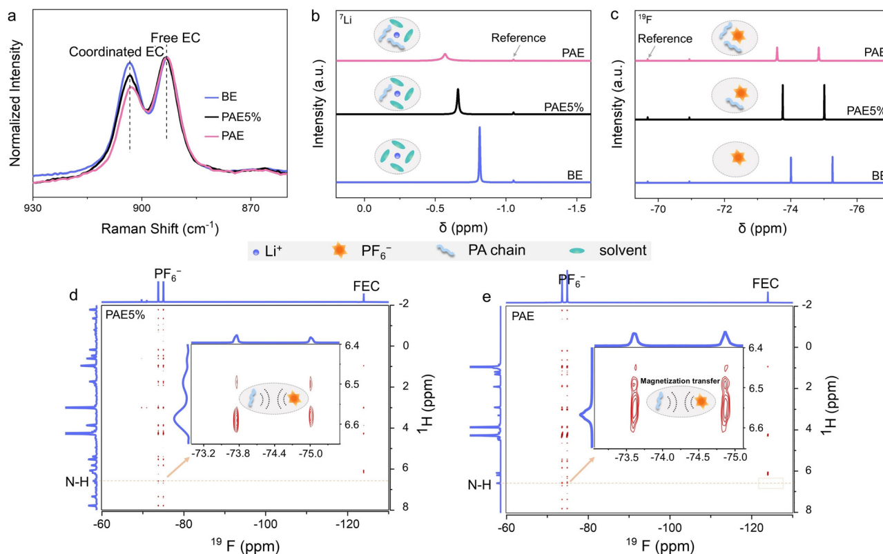
Fig. 3 Analysis of the nylon dissolution mechanism. (a) Raman spectra in the ranges of 860–930 \text{cm}^{-1} (the peak located at 893.2 \text{cm}^{-1} ). (b) ^7\text{Li} and (c) ^{19}\text{F} NMR spectra of various samples. 2D ^{19}\text{F} - ^1\text{H} HOESY spectra showing the interaction of F with H-nuclei in the electrolytes for (d) PAE 5% (BE with 5 wt% PA dissolved) and (e) PAE (BE with 10 wt% PA dissolved). The insets show the details of the cross signals between the H-nuclei of N–H groups and the F nuclei of \text{PF}_6^- anions. The external reference for the NMR spectra is 0.02 M \text{LiPF}_6 in a deuterated-DMSO (dimethyl sulfoxide- \text{d}_6 ) solution.
