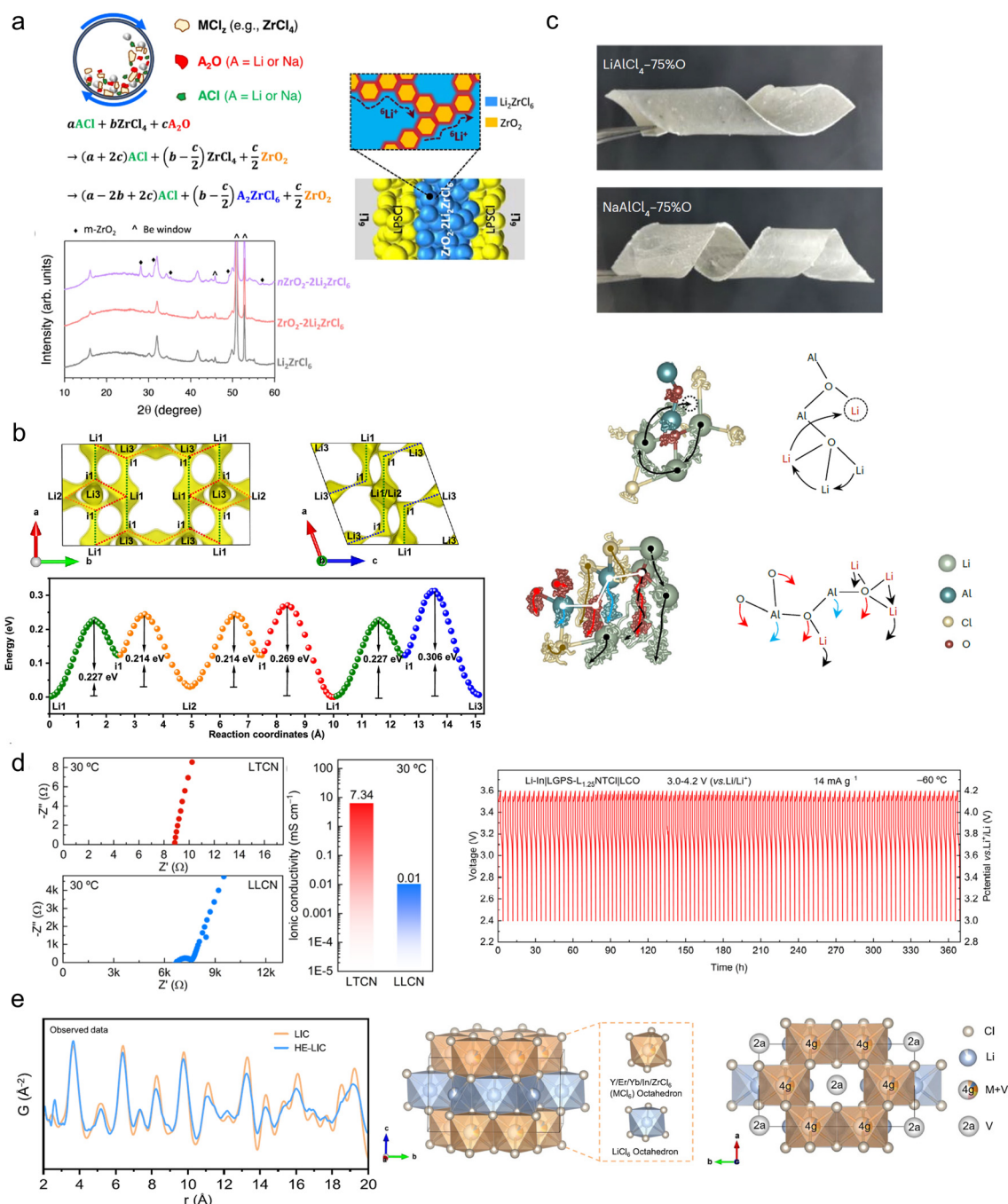
Fig. 5 (a) Preparation of \text{ZrO}_2(\text{-AlCl})\text{-A}_2\text{ZrCl}_6 ( \text{A} = \text{Li} or \text{Na} ) through a two-step ball-milling synthesis method, and the schematic diagram of the interfacial superionic \text{Li}^+ diffusion pathways. 101 (b) \text{Li}^+ migration pathways and migration energy barriers in \text{Li}_3\text{Zr}_{0.75}\text{OCl}_4 . 102 (c) The hopping and migration of \text{Li}^+ in the viscoelastic electrolytes LACO and NACO. 39 (d) The high ionic conductivity and excellent extremely low temperature performance of amorphous nitrogen-halide electrolytes \text{Li}_{3x}\text{TaCl}_5\text{N}_x . 105,106 (e) The local structure and unit cell of HE-LIC. 107
