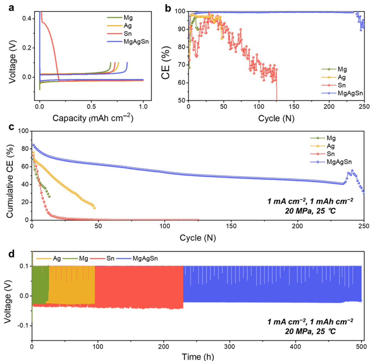
Fig. 2 Half-cell Li plating–stripping evaluations of the single- and multi-seed anode-less electrodes. (a) Voltage profiles of the first cycle. (b) Coulombic efficiencies (CEs), (c) cumulative CEs, and (d) voltage–time profiles of the half-cells over cycling.
