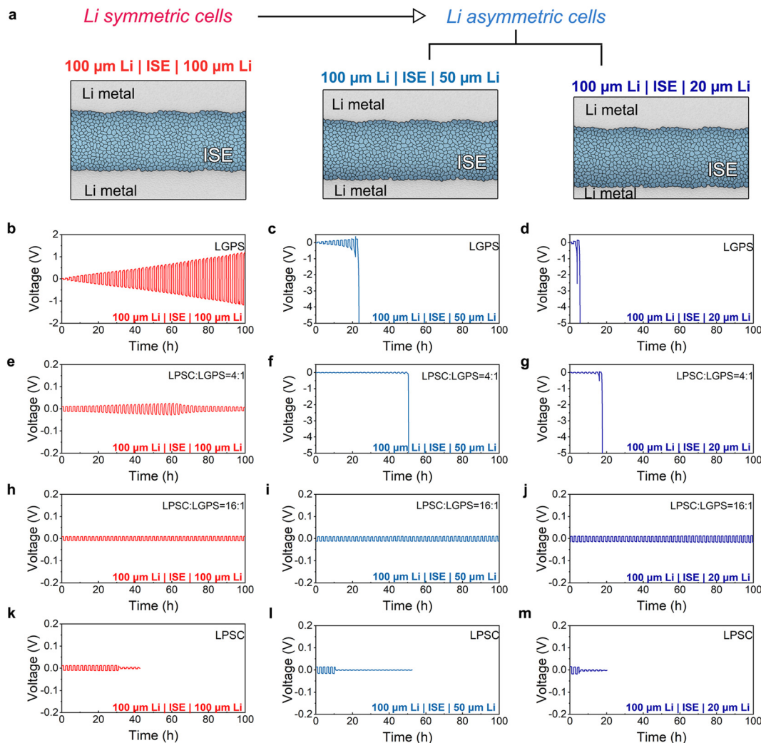
Fig. 2 (a) The schematic diagram of Li symmetric and asymmetric cells used in the evaluation. (b–d) Voltage profiles of the 100 μm thick Li | LGPS | 100 μm thick Li symmetric cell (b), 100 μm thick Li | LGPS | 50 μm thick Li (c) and 100 μm thick Li | LGPS | 20 μm thick Li asymmetric cells (d). (e–g) Voltage profiles of the 100 μm thick Li | LPSC : LGPS = 4 : 1 | 100 μm thick Li symmetric cell (e), 100 μm thick Li | LPSC : LGPS = 4 : 1 | 50 μm thick Li (f) and 100 μm thick Li | LPSC : LGPS = 4 : 1 | 20 μm thick Li asymmetric cells (g). (h–j) Voltage profiles of the 100 μm thick Li | LPSC : LGPS = 16 : 1 | 100 μm thick Li symmetric cell (h), 100 μm thick Li | LPSC : LGPS = 16 : 1 | 50 μm thick Li (i) and 100 μm thick Li | LPSC : LGPS = 16 : 1 | 20 μm thick Li asymmetric cells (j). (k–m) Voltage profiles of the 100 μm-thick Li | LPSC | 100 μm thick Li symmetric cell (k), 100 μm Li | LPSC | 50 μm thick Li (l) and 100 μm thick Li | LPSC | 20 μm thick Li asymmetric cells (m).
