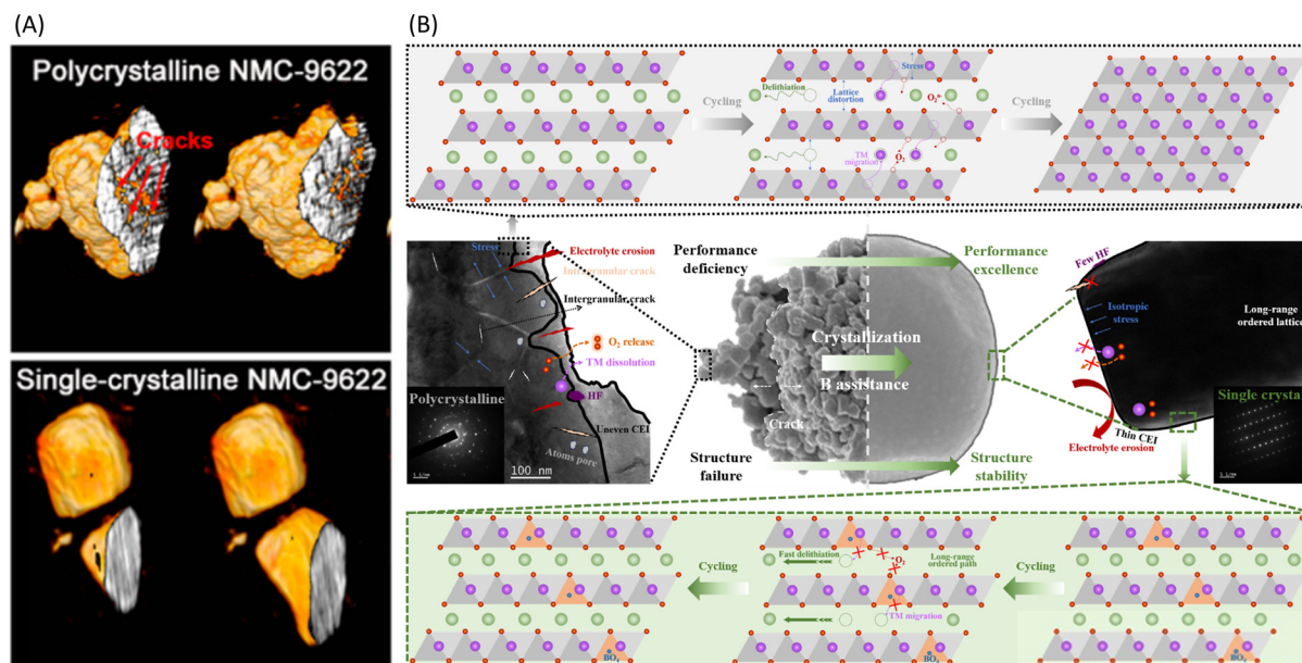
Fig. 14 (A) 3D tomographic reconstruction and multislicing analysis of a representative PC9622 and SC9622 secondary particle after long-term cycling. Reproduced with permission from ref. 126. Copyright 2021, American Chemical Society. SC9622, a novel single-crystalline ultrahigh-Ni layered cathode with a designed composition of \text{LiNi}_{0.96}\text{Mn}_{0.02}\text{Co}_{0.02}\text{O}_2 . PC9622, a baseline polycrystalline cathode with the same designed composition. (B) B-doped micron-sized single-crystal Co-free LRMO were obtained by molten-salt ( \text{LiNO}_3 and \text{H}_3\text{BO}_3 )-assisted sintering. Reproduced with permission from ref. 127. Copyright 2024, American Chemical Society.
