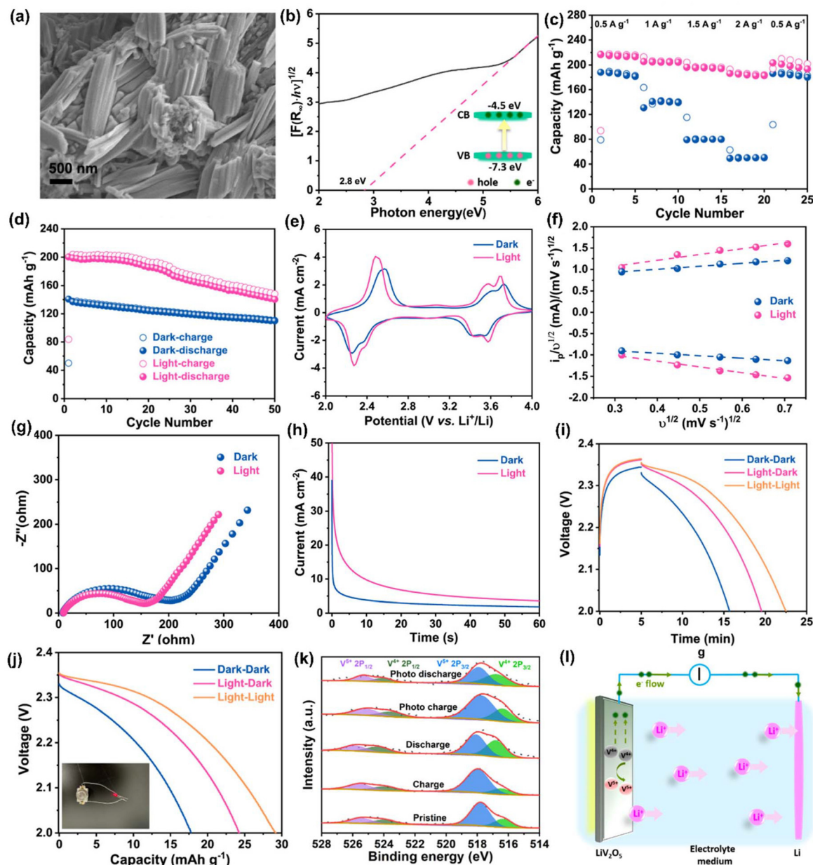
Fig. 7 (a) SEM image and (b) Kubelka–Munk curve from the diffusion reflectance spectra of LiV_2O_5 (inset: band energy diagram), (c) rate performance based on GCD curves at 0.5, 1.0, 1.5, and 2.0 A\text{ g}^{-1} in dark and light conditions, (d) cycling stability at 1.0 A\text{ g}^{-1} in dark and light conditions, (e) CV curves at 0.3 mV\text{ s}^{-1} , (f) diffusion constant analysis, (g) AC impedance spectra (h) J-t curves after charging at 2.5 V_{Li+/0} for 60 s in dark and under illumination, (i) photocharge and galvanostatic discharge curves, (j) corresponding discharge capacities (inset: photograph of a 2 V LED powered by a Li-ion PARB), (k) XPS spectra of V 2p_{3/2} and V 2p_{1/2} of LiV_2O_5 , (l) schematic illustration of the photoassisted charging mechanism of the Li-ion PARB. 38 Copyright: 2022 American Chemical Society.
