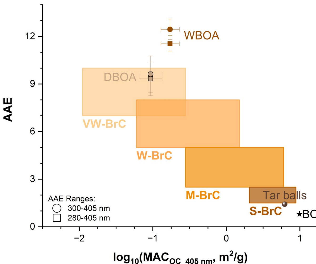
Figure 3. Classification of WBOA and DBOA mixtures according to the optical framework of Saleh 2020. 4 Average AAE and \log_{10}(\text{MAC}_{\text{OC}_{405 \text{ nm}}}) are calculated for the DBOA and WBOA samples. 44 AAE values are calculated over 280–405 nm (squares) and 300–405 nm (circles) spectral ranges. Reference values for BC 76 and strongly absorbing BrC 77 are included for visual comparison.
