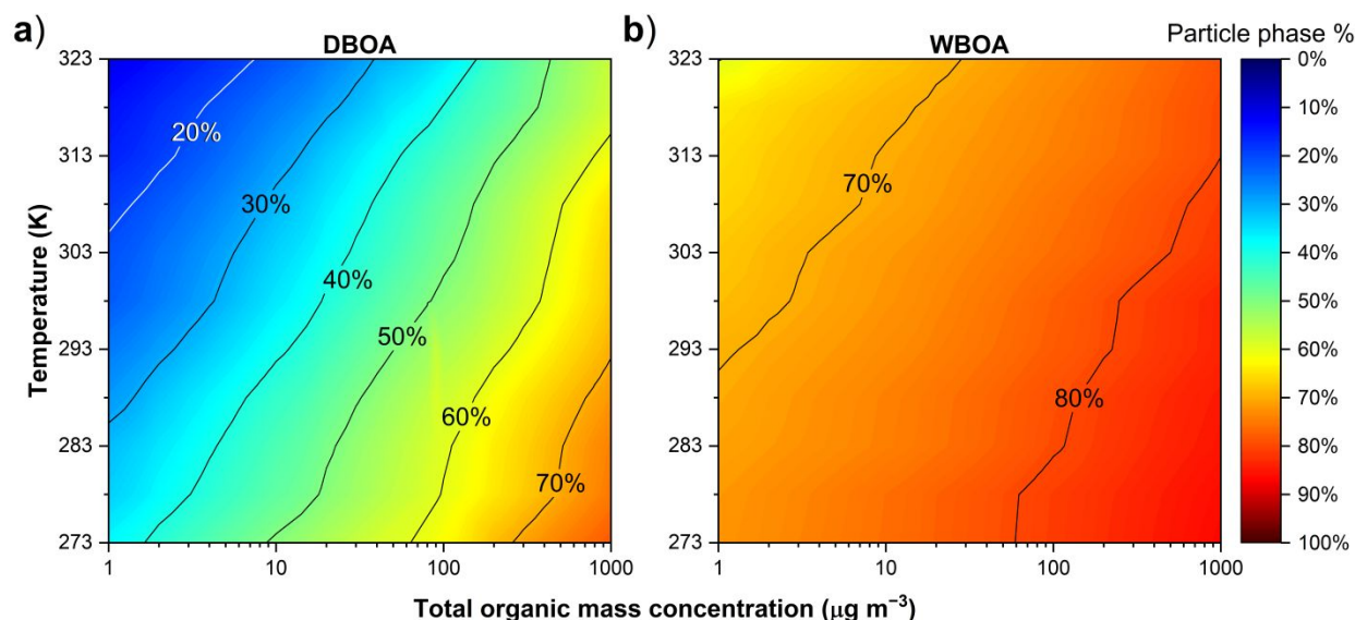
Figure 5. Calculated particle-phase mass fractions of (a) DBOA and (b) WBOA constituents as a function of tOM and T . Heatmap colors indicate the particle-phase mass fractions. The DBOA mixture shows a greater degree of gas-particle partitioning compared to WBOA, reflecting the higher volatility of its components relative to the less volatile species in the WBOA mixture.
