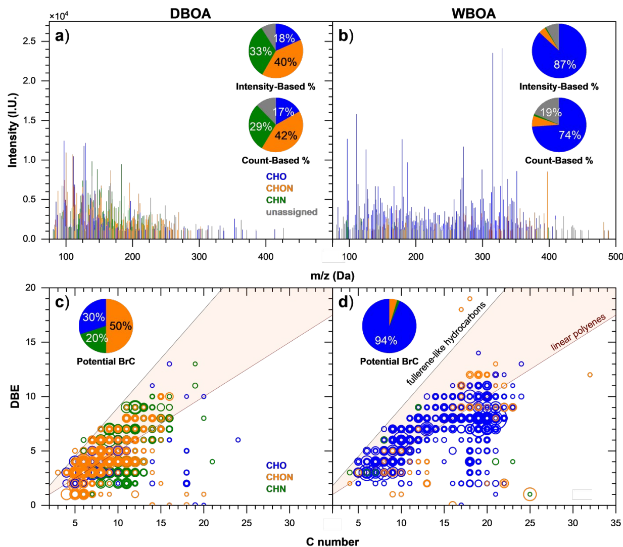
Figure 4. ESI(+) high-resolution mass spectra and DBE plots of DBOA (a, c) and WBOA (b, d) mixtures. Assigned compounds are color-coded by molecular class (CHO, CHN, CHON), with signal intensities and marker sizes scaled by the square root for better visualization. Pie charts represent the count-weighted and intensity-weighted abundances of molecular classes and unassigned species. In the DBE plots, compounds falling within the shaded region, bounded by the DBE ranges characteristic of fullerene-like hydrocarbons and linear polyenes, are potential BrC chromophores. Pie charts illustrate the relative abundance of potential BrC species resolved by compound class. The WBOA mixture is characterized by a dominant CHO composition, reflecting its lignin-rich nature of wood biomass, while the DBOA mixture is enriched in reduced N-containing species reflecting the composition of dung biofuel.
