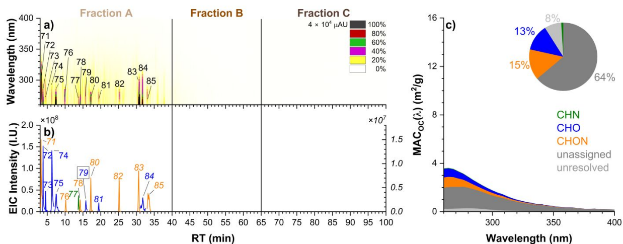
Figure 1. Characterization of major chromophoric compounds in the DBOA sample. (a) HPLC-PDA absorbance heatmap chromatogram, (b) HPLC-HRMS extracted ion chromatogram overlay, (c) fractional MAC_{Oc}(\lambda) contributions of major DBOA chromophores. Assigned PDA features are numbered in order of retention time and color-coded based on compound class. Italicized labels indicate MS features with intensities referenced to the right-hand axis; boxed labels denote BrC chromophores matched to compounds in the G1–G4 reference mixtures. Among the identified chromophores, CHON and CHN compounds contribute 16% of the total absorbance, followed by 13% contributed by CHO species.
