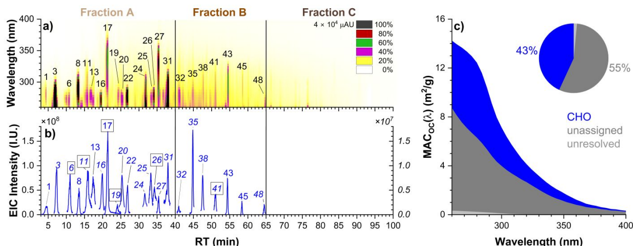
Figure 2. Characterization of major chromophoric compounds in the WBOA sample. (a) HPLC-PDA absorbance heatmap (b) HPLC-HRMS extracted ion chromatogram overlay, and (c) fractional MAC_{Oc}(\lambda) contributions of major WBOA chromophores. Assigned PDA features are numbered in order of retention time and color-coded based on compound class (CHO, blue). Italicized labels indicate MS features with intensities referenced to the right-hand axis; boxed labels denote BrC features matched to compounds in the G1–G4 reference libraries. Assigned CHO compounds contribute up to 43% of total absorbance.
