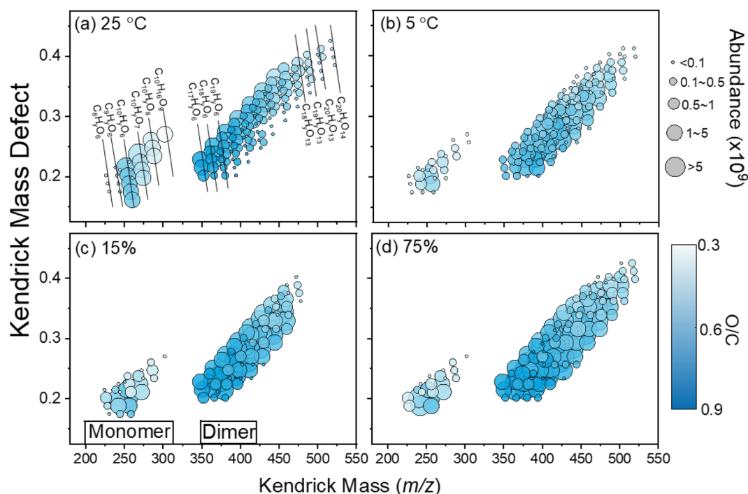
Fig. 4 Mass defect plot of HOM signals from limonene ozonolysis measured from (a) T = 25\text{ }^{\circ}\text{C} , (b) T = 5\text{ }^{\circ}\text{C} , (c) \text{RH} = 15\% , and (d) \text{RH} = 75\% .
