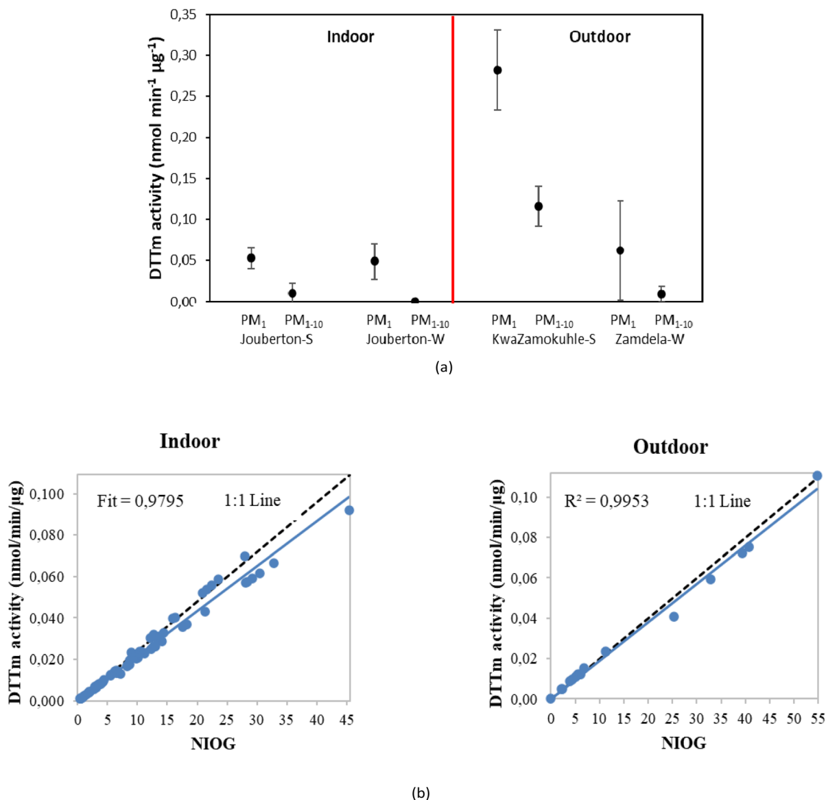
Fig. 8 (a) DTTm activity ( \text{nmol min}^{-1} \mu\text{g}^{-1} ) for PM nucleopore samples collected from Jouberton (summer and winter), KwaZamokuhle (summer) and Zamdela (winter) for PM 1 and PM 1-10 size fractions, and (b) correlation between DTTm activity and NIOG for outdoor and indoor samples.
