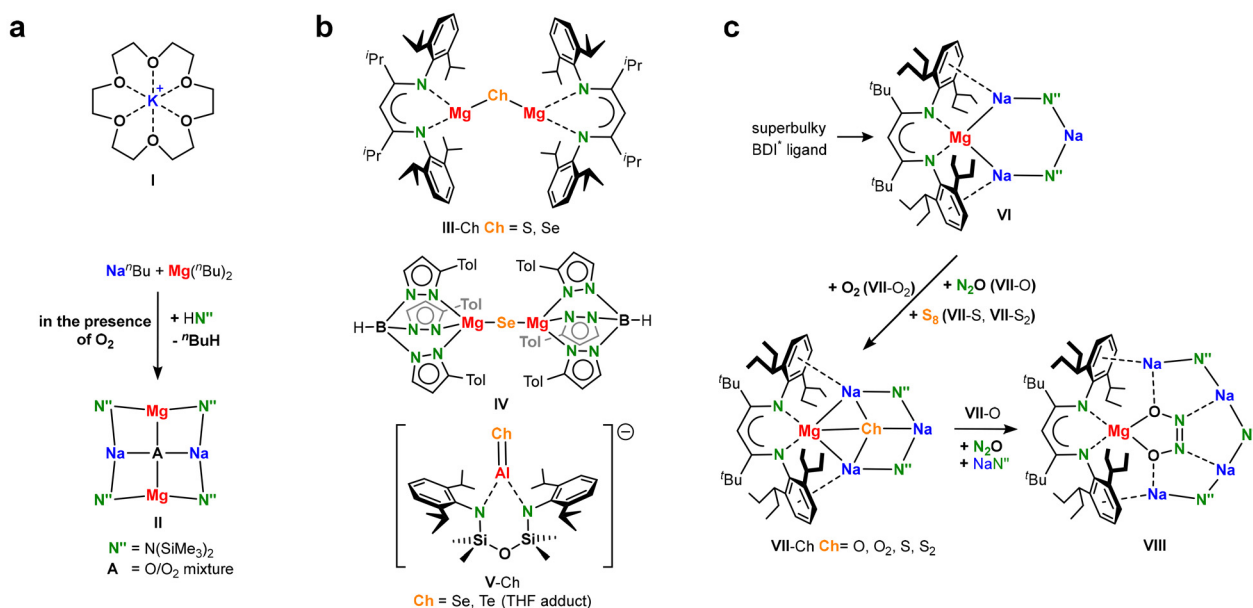
Scheme 1 (a) From Pedersen's crown ethers 1–3 to Mulvey's inverse crown complexes. 4–6 (b) Main group metal complexes with formal \text{Ch}^- centres. 8–11 (c) The reduction of \text{O}_2 , \text{N}_2\text{O} or \text{S}_8 with redox-active metal crown complex VI . 24
