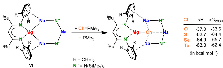
Scheme 2 Calculated reaction enthalpies and free energies (kcal mol −1 ; B3PW91-GD3BJ/def2tzvp//B3PW91-GD3BJ/def2svp) for reaction of VI with \text{Me}_3\text{P}=\text{Ch} to metal crown complexes of the \text{Ch}^{2-} anions.
