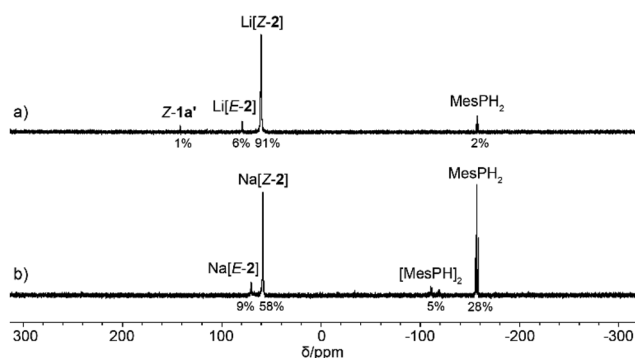
Fig. 2 ^{31}\text{P} NMR spectrum (162 MHz, THF) of the reaction mixture for the synthesis of (a) \text{Li}[Z-2]\cdot\text{THF} and (b) \text{Na}[Z-2]\cdot\text{THF} .
