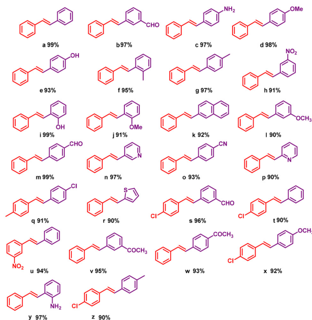
Scheme 7 Substrate scope Heck-coupling reaction. Conditions: aryl chloride (0.50 mmol), styrene (0.60 mmol), \text{Cs}_2\text{CO}_3 (0.60 mmol), DMF 2 mL, 120 °C, and catalyst 1 (0.1 mol%). All are isolated yields.
