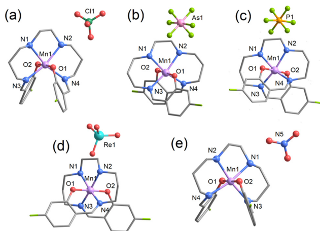
Fig. 1 The crystal structures of complexes 1 (a), 2 (b), 3 (c), 4 (d), and 5 (e) at 300 K. Color code: Mn, bright purple; C, grey; N, blue; O, red; F, pale yellow; Cl, green; As, pink; P, orange; Re, sky blue. Hydrogen atoms are omitted for clarity.
