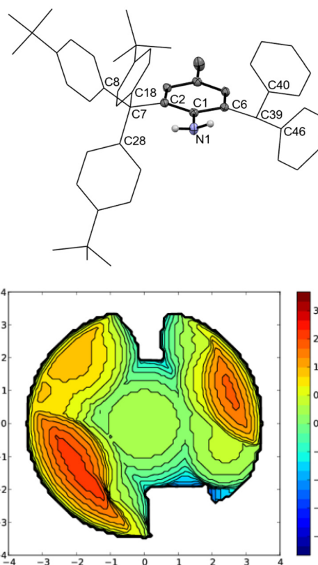
Fig. 1 The molecular structure (above) and the steric map 33 (below) of 1 . An ORTEP diagram, 40% probability level. The shielding groups are displayed as wireframes for clarity. Selected interatomic distances [Å] and angles [°]: C1–N1 1.4031(19), C2–C7 1.5561(18), C7–C28 1.546(2), C6–C39 1.5295(19), C39–C40 1.531(2).
