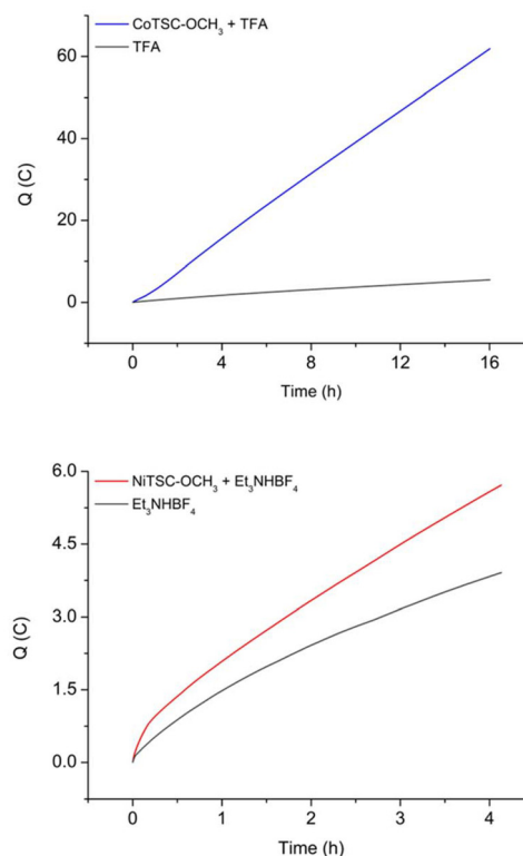
Fig. 2 Coulometry of CoTSC- \text{OCH}_3 with 60 mM TFA during bulk electrolysis experiment at -1.6 V vs. \text{Fc}^{+/0} (top blue line) and blank experiment of 60 mM TFA in the absence of CoTSC- \text{OCH}_3 (top grey line) and NiTSC- \text{OCH}_3 with 100 mM \text{Et}_3\text{NHBF}_4 during bulk electrolysis experiment at -2.1 V vs. \text{Fc}^{+/0} (bottom red line) and blank experiment of 100 mM \text{Et}_3\text{NH}^+ in the absence of NiTSC- \text{OCH}_3 (bottom grey line). The electrolytic solutions contain 0.1 M \text{NBu}_4\text{PF}_6 in DMF and 1 mM of each complex. Bulk electrolysis experiments were performed using a mercury pool working electrode.
