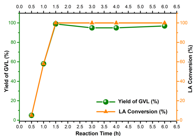
Fig. 7 The effect of the reaction time on the conversion of LA into GVL catalyzed by MO-Ru. Reaction conditions: MO-Ru (0.098 mmol, based on Ru content), LA (9.8 mmol), formic acid (19.6 mmol), H 2 O (4 mL), LA : FA ratio 1 : 2.
