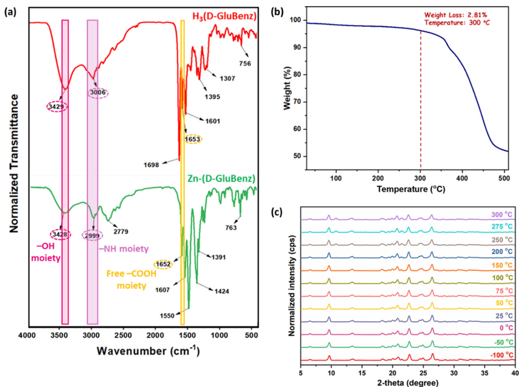
Fig. 1 (a) Comparison of FTIR spectra of H_3(D-GluBenz) and Zn-(D-GluBenz) , highlighting the catalytic sites, (b) thermogravimetric analysis profile and (c) VT PXRD patterns from -100 to +300 ^{\circ}C of Zn-(D-GluBenz) .
