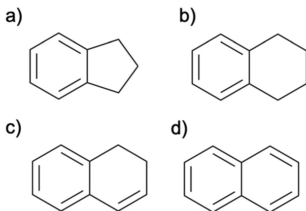
Fig. 1 Relevant structures on the path from polymethylbenzenes to naphthalenes. For simplicity, the unmethylated structures are shown. a) 2,3-dihydro-1H-indene b) 1,2,3,4-tetrahydronaphthalene c) 1,2-dihydronaphthalene d) naphthalene.
