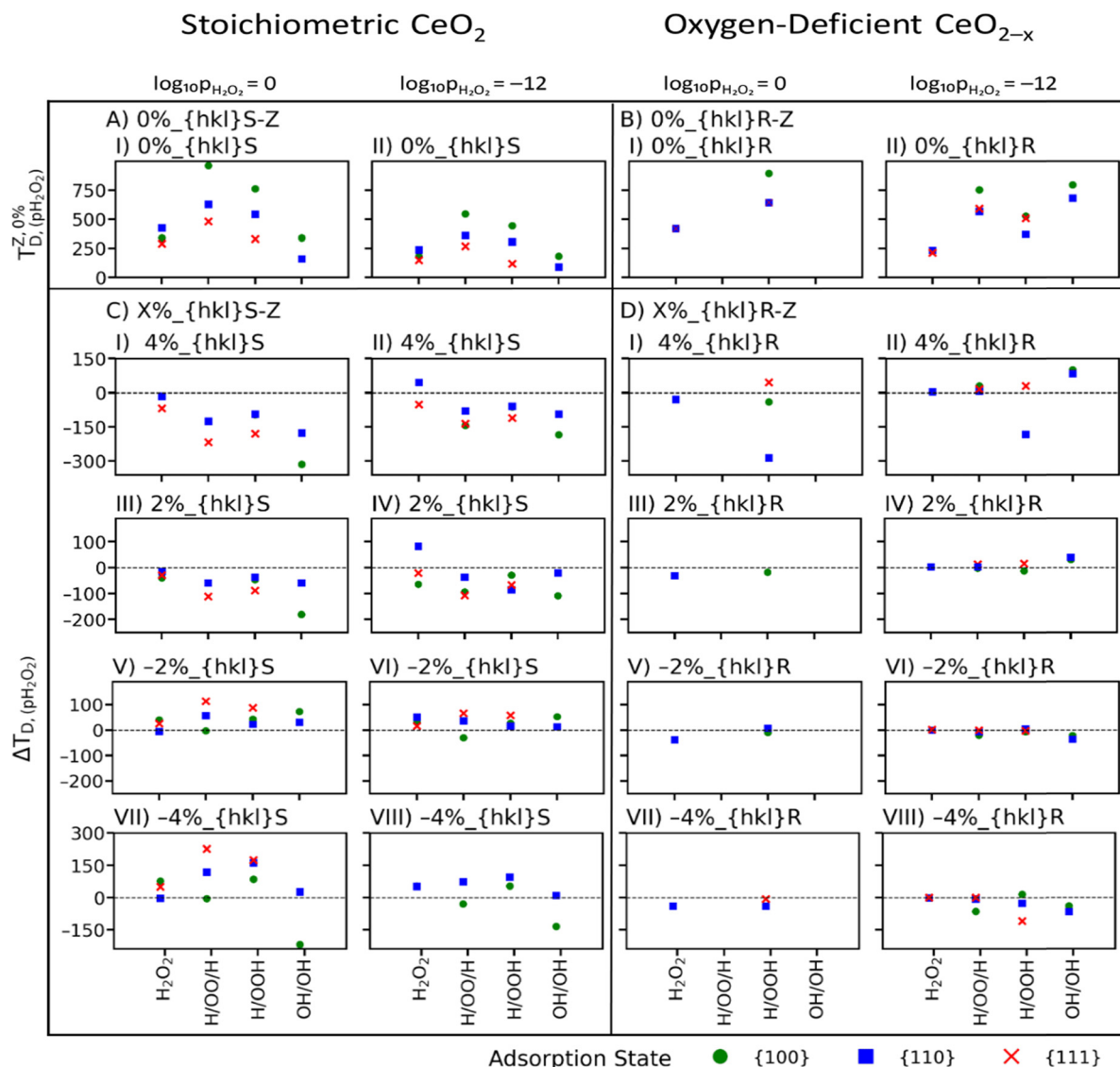
Fig. 3 Desorption temperature of molecularly and dissociatively adsorbed hydrogen peroxide on stoichiometric and oxygen-deficient CeO_2 . T_D^{N,0\%} of adsorbed hydrogen peroxide species on unstrained stoichiometric (A) and oxygen-deficient (B) CeO_2 surfaces. \Delta T_{D,(p_{H_2O_2})} of adsorbed hydrogen peroxide species on strained stoichiometric (C) and oxygen-deficient (D) CeO_2 surfaces.
