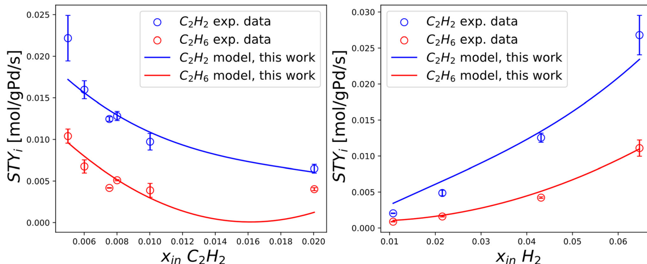
Fig. 8 Experimentally measured and modelled space-time yields of C_2H_2 and C_2H_6 ( STY_{C_2H_2} [mol g Pd -1 s -1 ] and STY_{C_2H_6} [mol g Pd -1 s -1 ]) plotted against single manipulated operating variables. Includes experimental data by Urmes et al. and model simulation results by this work. Left) Trends vs. inlet molar fraction of C_2H_2 obtained at 323 K, i.e. 50 °C. Right) Trends vs. inlet molar fraction of H_2 obtained at 323 K, i.e. 50 °C. The standard deviation of experimental measurements is reported through error bars for points whose reproducibility has been verified through at least two repeated experiments.
