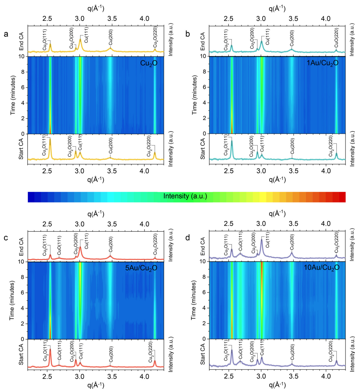
Fig. 4 Evolution of the X-ray diffractograms during the chronoamperometry measurement at -0.9 V vs. RHE for (a) \text{Cu}_2\text{O} , (b) 1\text{Au}/\text{Cu}_2\text{O} , (c) 5\text{Au}/\text{Cu}_2\text{O} and (d) 10\text{Au}/\text{Cu}_2\text{O} .
