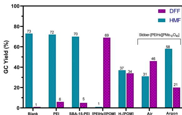
Fig. 6 Blank reaction comparison with \text{SiO}_2\text{-[PEIH]}_x\text{[POM]} in D-fructose valorisation. Reaction conditions: 200 mg of D-fructose (1.11 mmol), silica materials: 11.25 wt% (22.5 mg) of material for SBA-15-[PEIH] x [PMo 12 O 40 ] (0.06 mol% [PMo 12 O 40 ], 0.7 mol% Mo), for Stöber-[PEIH] x [PMo 12 O 40 ] (0.05 mol%, PMo 12 O 40 , 0.6 mol% Mo), for H 3 [PMo 12 O 40 ] and hybrid [PEIH] x [POM] materials (0.9 mol% POM), and 6 mL of DMSO, 150 °C, 5 h, in air. Yields of 5-HMF and DFF were determined by GC-FID employing naphthalene as the internal standard with \pm 4\% variability. Full conversion of fructose after 1 h was checked by 1 H NMR spectroscopy.
