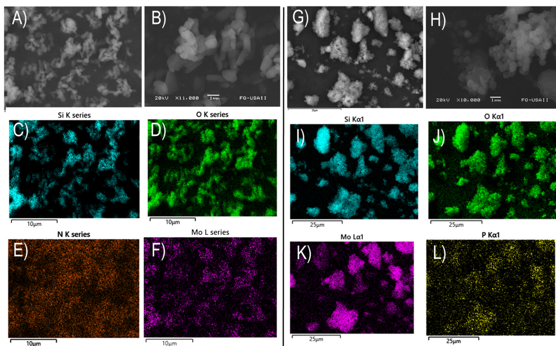
Fig. 2 SEM micrographs of as-synthesized materials. SBA-15-[PEIH] x [PMo 12 O 40 ] (low-magnification (A), high-magnification (B), EDS element mapping of Si (C), O (D), N (E) and Mo (F) and Stober-[PEIH] x [PMo 12 O 40 ] (low-magnification (G), high-magnification (H), EDX element mapping of Si (I), O (J), Mo (K) and P (L)).
