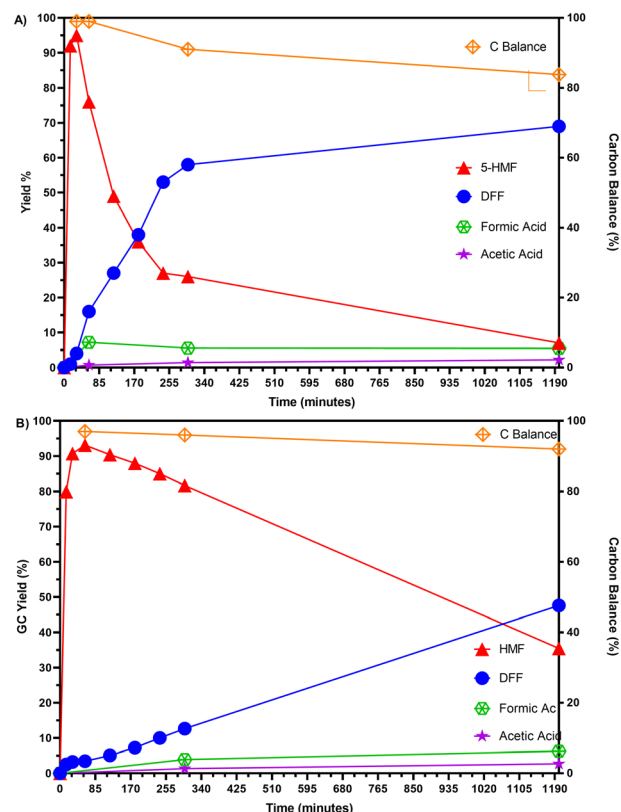
Fig. 7 The distribution of products versus reaction time employing A) Stöber-[PEIH x ] 2 [PMO 12 O 40 ] or B) SBA-15-[PEIH x ] 2 [PMO 12 O 40 ] in valorisation of D-fructose. Reaction conditions: 200 mg of D-fructose (1.11 mmol), 45 mg of Stöber or SBA-15-[PEIH x ] 2 [PMO 12 O 40 ] (22.5 wt%, 0.10 mol%, PMO 12 O 40 , 1.2 mol% Mo), 6 mL of solvent, 65 mg of naphthalene as the internal standard. HMF and DFF yields were determined by GC-FID; the acid concentration was determined by 1 H NMR (400 MHz) using naphthalene as the internal standard.
