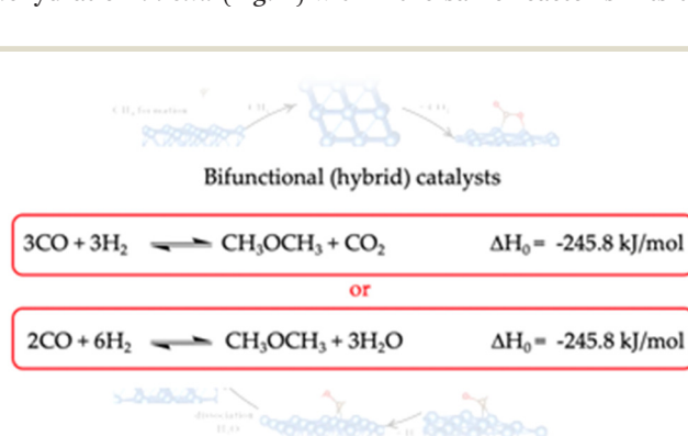
Fig. 2 Alternative (direct) one-step process DME synthesis.
