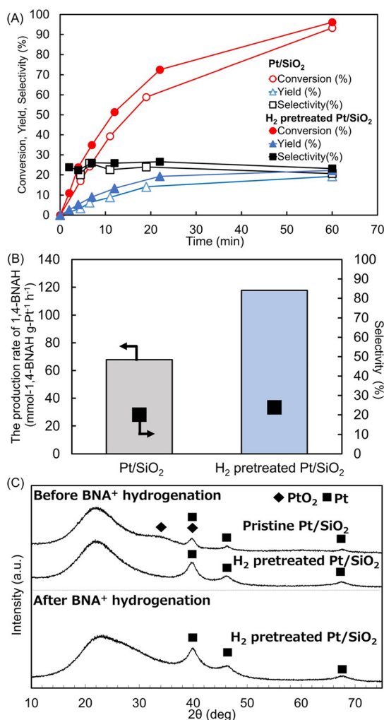
Fig. 5 (A) Time course of \text{BNA}^+ hydrogenation using Pt/ \text{SiO}_2 catalyst and \text{H}_2 -pretreated Pt/ \text{SiO}_2 catalyst. The reaction conditions: \text{BNA}^+ (1.5 mmol \text{L}^{-1} ) in 20 mL of 0.1 mol \text{L}^{-1} Tris-HCl buffer (pH 8.8) with a 4 wt% Pt/ \text{SiO}_2 catalyst (5 mg) at 20 °C under 1 atm \text{H}_2 . (B) Comparison of the 1,4-BNAH production rates. (C) XRD patterns of the 4 wt% Pt/ \text{SiO}_2 catalyst comparing of pristine, without \text{H}_2 pretreated, and \text{H}_2 pretreated samples at before (upper) and after (lower) \text{BNA}^+ hydrogenation.
