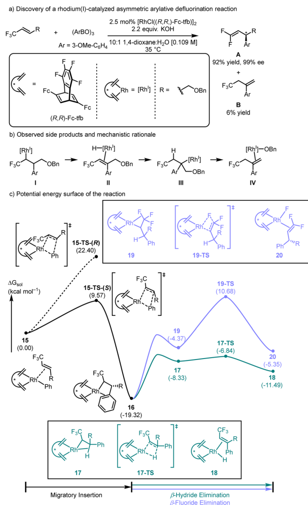
Scheme 5 (a) Enantioselective rhodium-catalyzed arylation-defluorination reaction of trifluoromethyl olefins and (b) β-hydride elimination pathway accounting for side product formation. (c) Reaction coordinate for the enantioselective defluorinative arylation developed by Hayashi in 2016. 31
