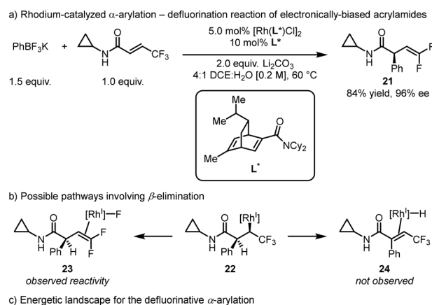
Scheme 5 (a) Enantioselective rhodium-catalyzed arylation-defluorination reaction of trifluoromethyl olefins and (b) β-hydride elimination pathway accounting for side product formation. (c) Reaction coordinate for the enantioselective defluorinative arylation developed by Hayashi in 2016. 31
