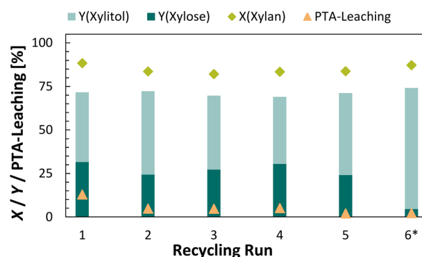
Fig. 2 Xylan conversion X , xylitol yield Y and PTA-leaching in the recycling of Ru_PTA/CTF3 hydrolytic hydrogenation of xylan. *4 h reaction time in 6th run (conditions: 130^\circ\text{C} , 2 h, 50 bar \text{H}_2 , 750 rpm, m(\text{xylan}) = 0.115 \text{ g} , m(\text{Ru_PTA/CTF-2}) = 140 \text{ mg} , V(\text{H}_2\text{O}) = 5 \text{ mL} ).
