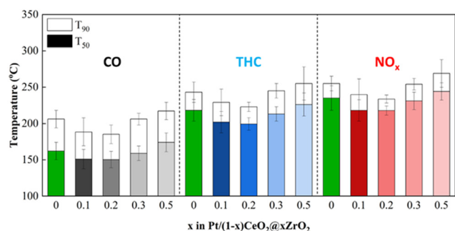
Fig. 6 Comparison of T_{50,90} s of CO, THCs and \text{NO}_x over DG 1.8 wt% \text{Pt}/(1-x)\text{CeO}_2@x\text{ZrO}_2 ( x = 0, 0.1, 0.2, 0.3, 0.5 ) catalysts; each bar represents the average T_{50,90} s of three different batches of the catalyst and the error bars represent the standard deviation of the T_{50,90} s.
