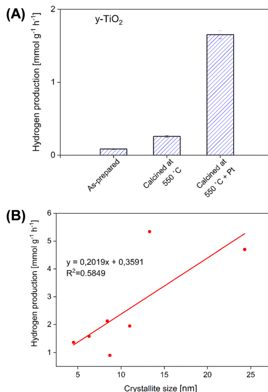
Fig. 2 (A) Hydrogen production rate of the prepared \gamma-TiO_2 catalysts and (B) relationship between crystallite size and hydrogen production.
