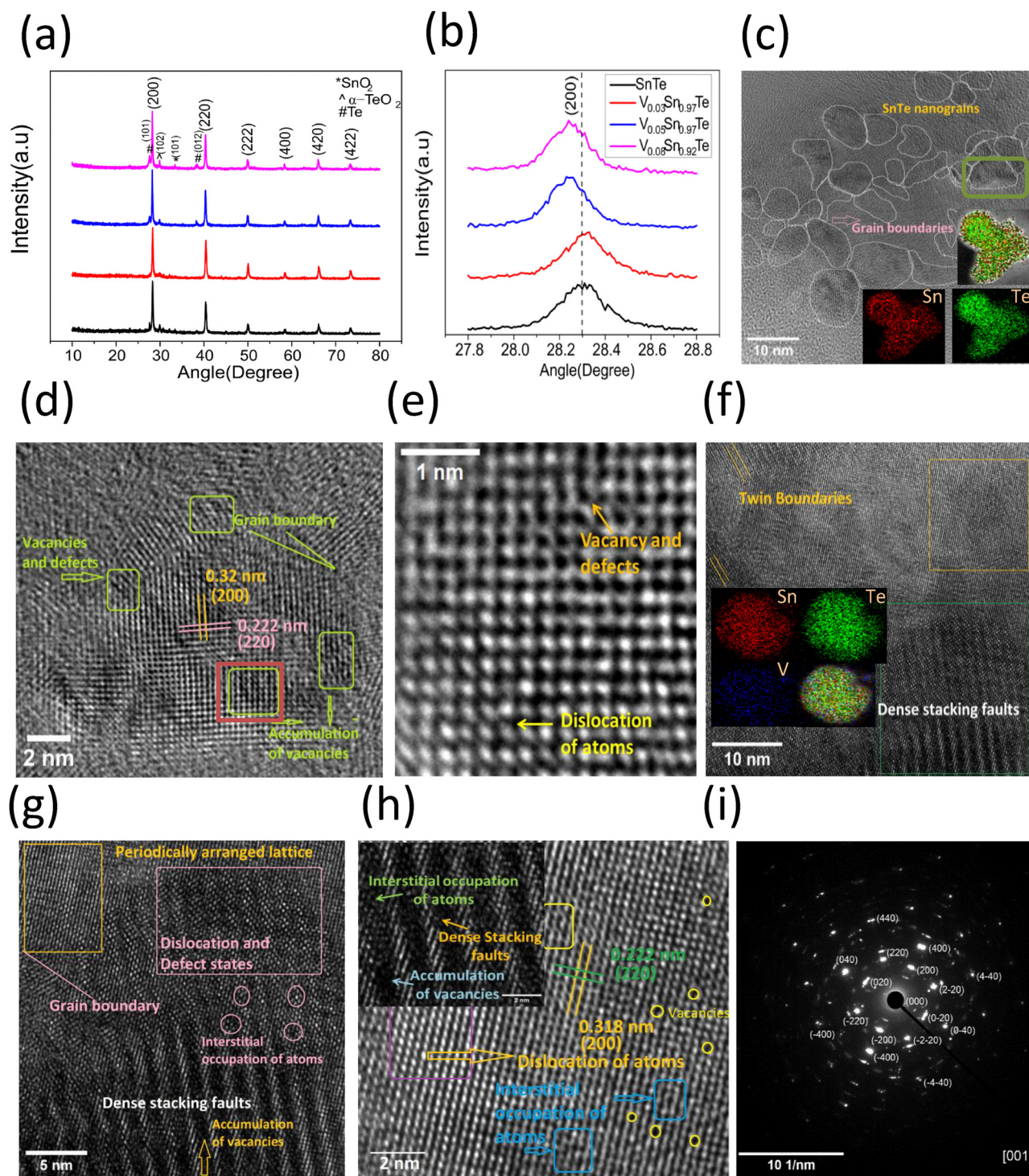
Fig. 1 (a) XRD and (b) enlarged view of the (200) plane of SnTe and V_x\text{Sn}_{1-x}\text{Te} ( x = 0.03, 0.05, 0.08 ). (c) HRTEM image of SnTe nanograins; white encloser regions show SnTe nanograins and the corresponding grain boundaries (insets show the HRTEM EDX elemental mappings of Sn, Te, and SnTe, respectively, with 50 nm scale bar). (d) The enlarged view of the larger grain (enclosed by the green rectangle) shows the interplanar spacing of the (200) and (220) planes, grain boundaries, vacancies, defects, and accumulation of vacancies in different green rectangular enclosed regions. (e) The SAED pattern of bare SnTe. (f) HRTEM image of V_{0.03}\text{Sn}_{0.97}\text{Te} nanograins of 47.32 nm diameter shows twin boundaries, dense stacking faults, and various defect states (insets show the HRTEM EDX elemental mappings of Sn, Te, V, and V_{0.03}\text{Sn}_{0.97}\text{Te} , respectively, with 25 nm scale bar). (g) The enlarged view of the larger grain (enclosed by the yellow rectangle) shows the interplanar spacing of the (200) and (220) planes, vacancies, defects, dislocation, and interstitial occupation of atoms. (h) The enlarged view of the larger grain (enclosed by the green rectangle) shows dense stacking faults, accumulation of vacancies, interstitial occupation of atoms, grain boundary, dislocation, and defect states. (i) SAED pattern of V_{0.03}\text{Sn}_{0.97}\text{Te} .
