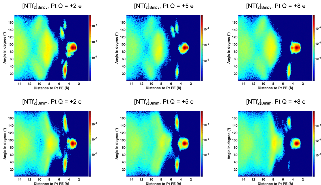
Fig. 9 IL anion orientation distribution near the Pt PE region: [NTf 2 ] Bmpy (top row) vs. [NTf 2 ] Bmim (bottom row), under different Pt electrode charge conditions.
