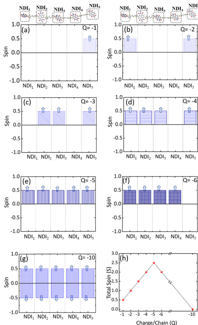
Fig. 5 The electronic spin distribution on individual NDI-units within the NDI-TVTV polymer chain showing distinct spin states at all the reduction levels in the solvent phase (water). (a) Q = -1 , (b) Q = -2 , (c) Q = -3 , (d) Q = -4 , (e) Q = -5 , (f) Q = -6 , and (g) Q = -10 . (h) The electronic total spin ( S ) of the PNDI-TVTV chain at different charged states in the solvent phase (water).
