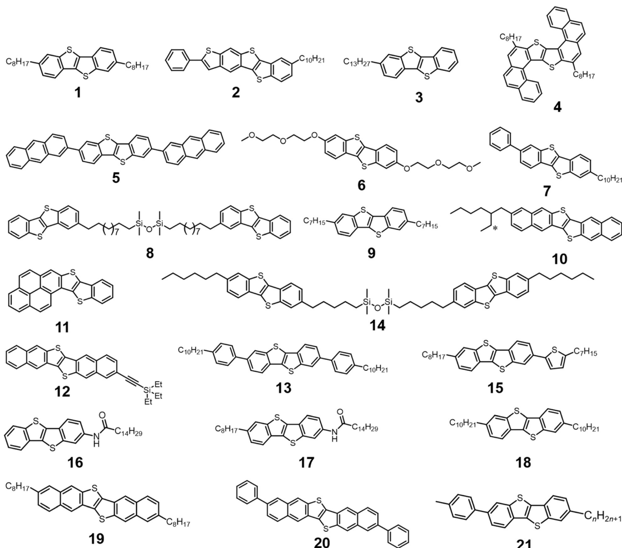
Fig. 3 Molecular structures of BTBT derivatives reported in recent studies.
