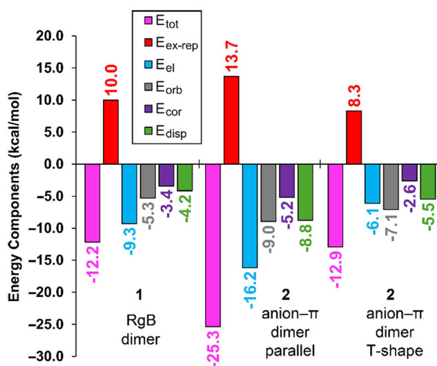
Fig. 12 The total, E_{tot} (pink); exchange repulsion, E_{ex-rep} (red); electrostatic, E_{el} (blue); orbital, E_{orb} (grey); correlation, E_{cor} (purple) and dispersion, E_{disp} (green) energies for the RgB dimer of compound 1 and the two \pi -stacking modes of compound 2.
