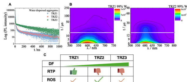
Fig. 3 (A) Fluorescence kinetics obtained via TC-SPC for TRZ1–3 in water dispersion (99%W). (B) TRES matrix in the microsecond time range for TRZ1–2 aggregates in a water dispersion. (C) Sketch of the DF, RTP, and ROS generation revealed for TRZ1–3 .
