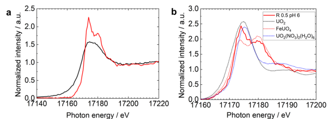
Fig. 1 (a) U L 3 edge HERFD-XANES spectrum (red line) and XANES spectrum (black line) of U-magnetite samples prepared at pH 6. (b) (Solid line) U L 3 edge HERFD-XANES spectrum of U-magnetite samples prepared at pH 6. (Dotted line) HERFD-XANES spectra of UO 2 (black), FeUO 4 (red), and UO 2 (NO 3 ) 2 ·6H 2 O (blue), previously published by Yomogida et al. 28
