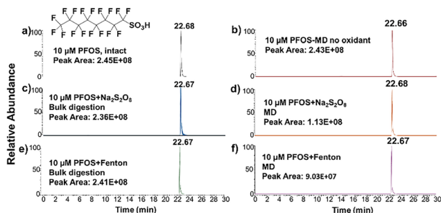
Fig. 3 EIC of the signal [PFOS-H]^- of 10 \mu M PFOS (a) before degradation, (b) after degradation in microdroplets without oxidant additive, (c) after degradation in bulk solution using S_2O_8^{2-} additive, (d) after degradation in microdroplets containing S_2O_8^{2-} , (e) after degradation in bulk solution using Fenton's reagent additive, and (f) after degradation in microdroplets containing Fenton's reagent.
