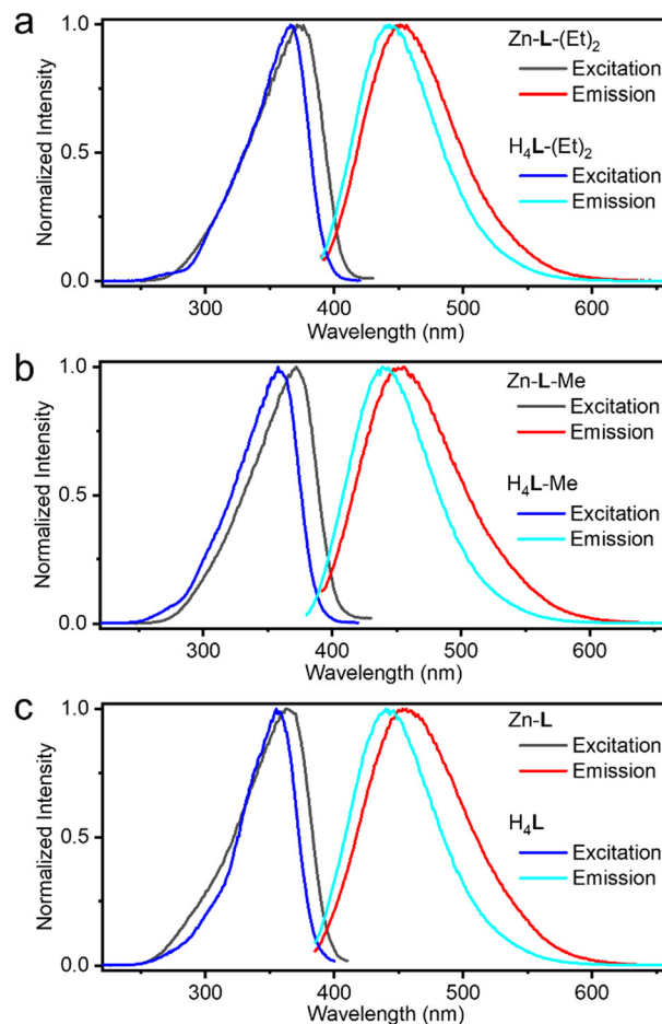
Fig. 2 Excitation and emission spectra of CMOFs and ligands, (a) \text{Zn-L}(\text{Et})_2 and \text{H}_4\text{L}(\text{Et})_2 , (b) \text{Zn-L-Me} and \text{H}_4\text{L-Me} , (c) \text{Zn-L} and \text{H}_4\text{L} .
