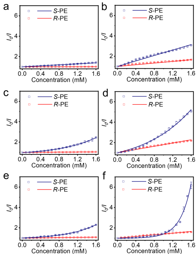
Fig. 3 Stern-Völmer plots (points for data and lines for fitting) for \text{H}_4\text{L}-(\text{Et})_2 (a), \text{Zn-L}-(\text{Et})_2 (b), \text{H}_4\text{L-Me} (c), \text{Zn-L-Me} (d), \text{H}_4\text{L} (e) and \text{Zn-L} (f) with increasing concentrations of R-PE and S-PE.
