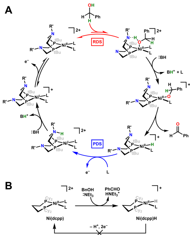
Fig. 3 (A) Catalytic cycle for Ni(P 2 N 2 ) based on the most recent mechanistic study from Gunasekara et al. (:B = NEt 3 , L = MeCN, R' = tBu, Ph, Bn) (B) Structure of Ni(dc 2 pp) control catalyst demonstrating inaccessibility of catalyst regeneration without the pendent amine.
