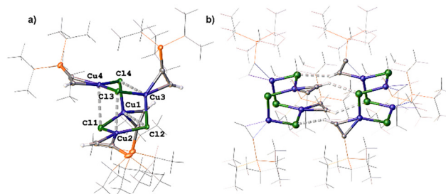
Fig. 2 Solid-state structure of ( 1 ). (a) The \text{Cu}_4\text{Cl}_4 -core and \text{SiCCH} drawn as thermal ellipsoids (50% probability levels); \text{iPr} -groups are rendered as wire frame for clarity. (b) Weak hydrogen bonding ( \text{CC-H}\cdots\text{Cl} ) linking clusters of 1 into a 1D-network.
